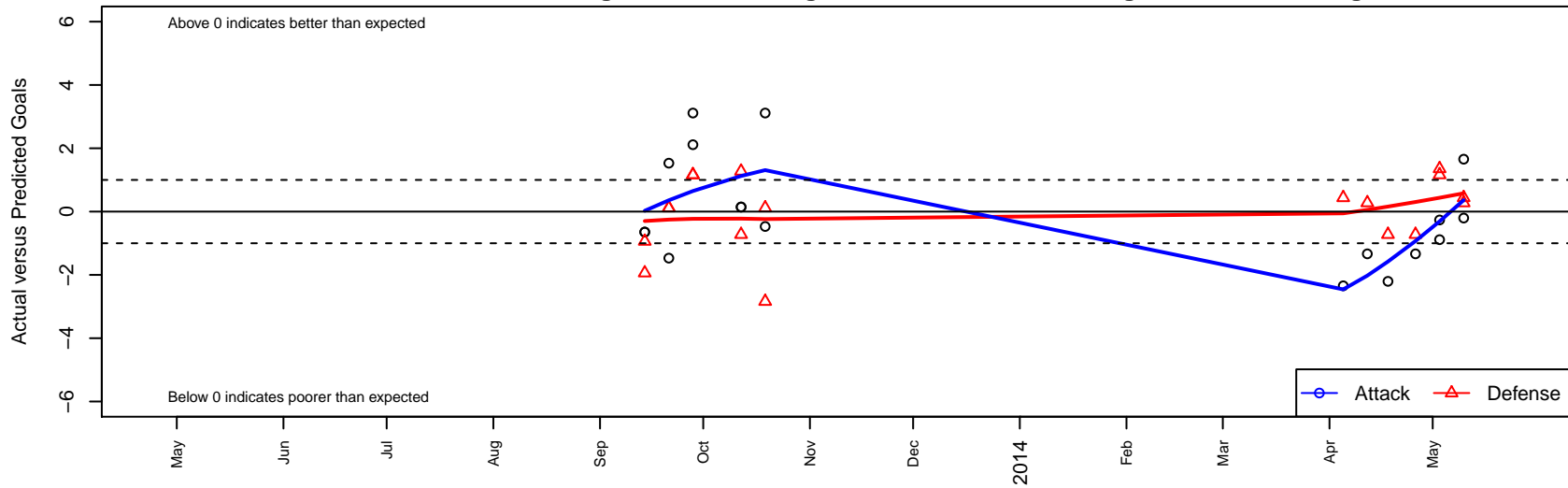
Union Couny United G01 Dots are actual minus expected GF (blue circles) and GA (red triangles). Blue line is smoothed change in attack strength. Red is smoothed change in defense strength.
